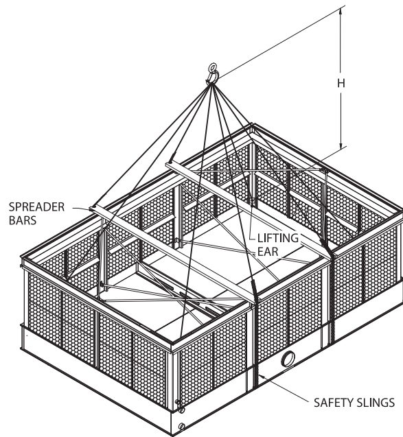
Figure 7 - Extended Lifts
