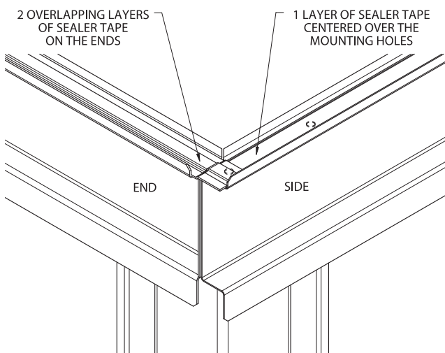
Figure 5a - Sealer Tape on Flange of Basin Section
