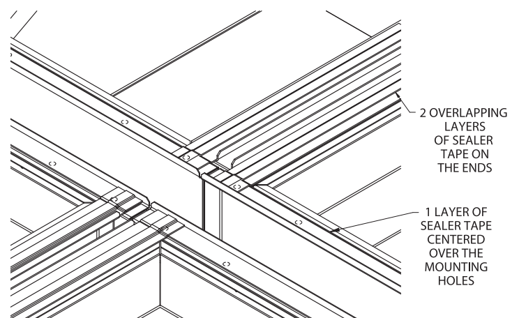
Figure 5b - Sealer Tape Detail for Center Joint of Units with Four Top (Coil/ Fan) Sections
