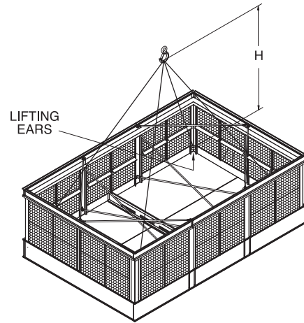
Figure 1a - Basin Section up to 21' (6.4m) long
