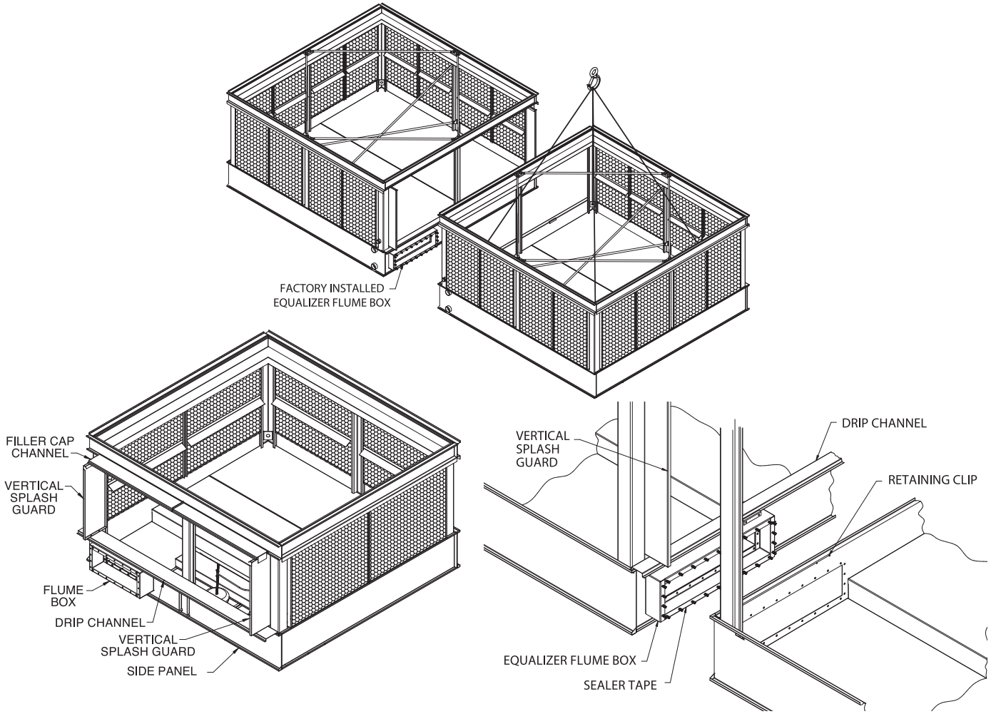
Figure 3 - Joining Bottom Sections – Multi Cell Units
