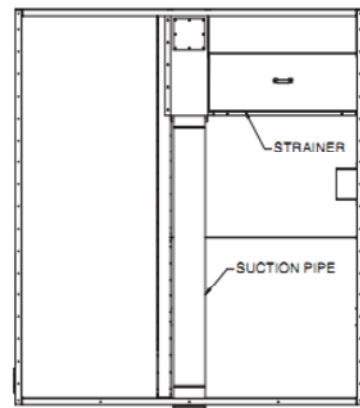
Figure 12b – Strainer Location on 2.5m Wide Units.
