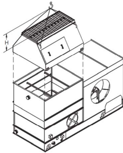
Figure 6b – Rigging Tapered Discharge Hood
