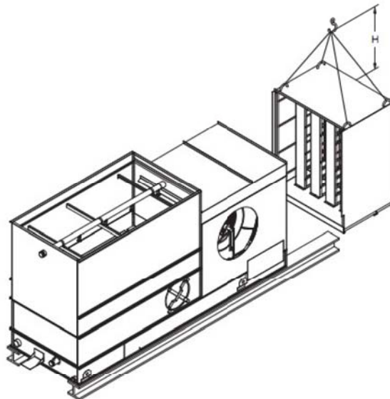
Figure 8 – Rigging Fan-End Sound Attenuator Assembly
