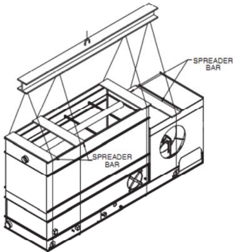
Figure 3a – Recommended Safety Sling Rigging
