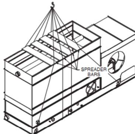
Figure 3b – Alternative Safety Sling Rigging
