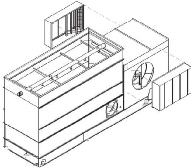
Figure 10 – Rigging Fan-Side Sound Attenuator Assembly
