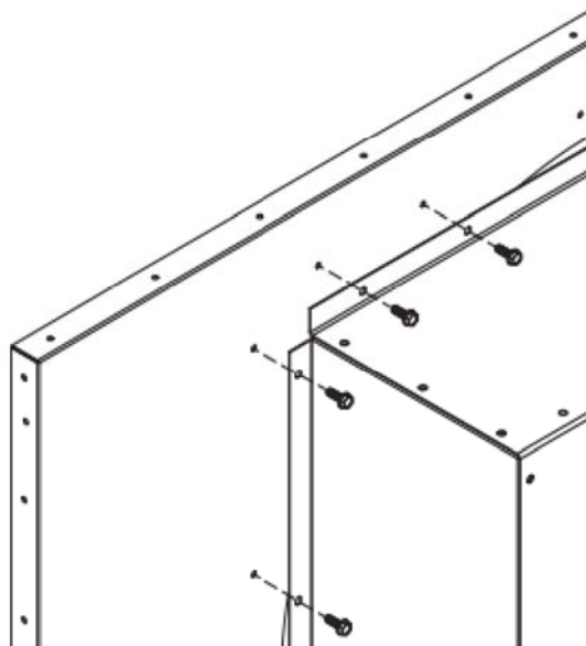
Figure 11 – Fan-Side Sound Attenuator Assembly Details
