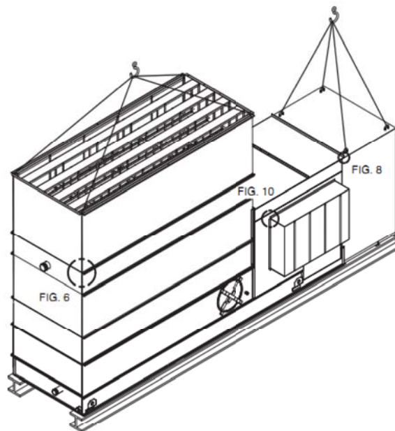
Figure 5 – Discharge and Intake Accessory Rigging
