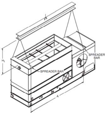
Figure 2a – Recommended Rigging - LP/LR Main Unit
