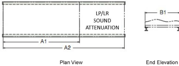
Figure 1 – Structural Steel Support
