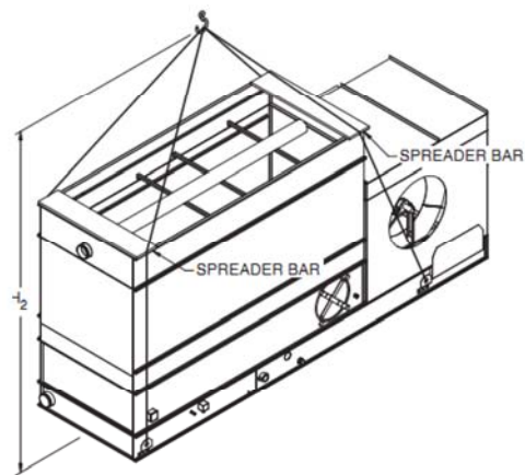
Figure 2b – Alternate Rigging - LP/LR Main Unit
