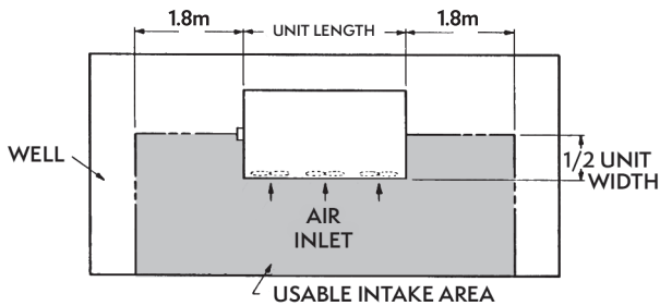
Figure 46 – Well Installation
