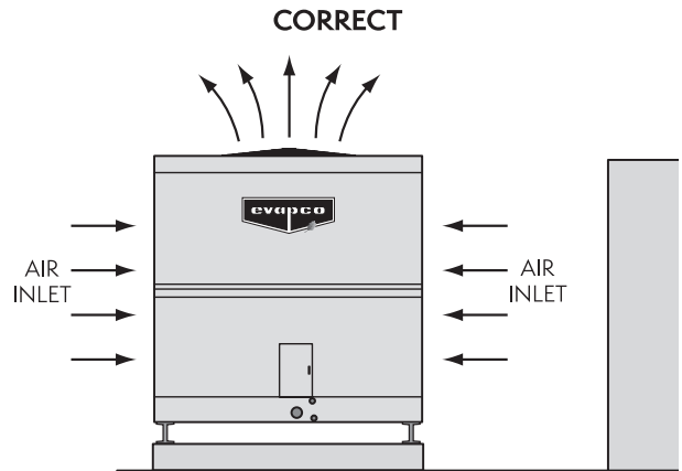
Figure 25 – Installation Elevated so Top of Unit Is Higher than Top of Wall
