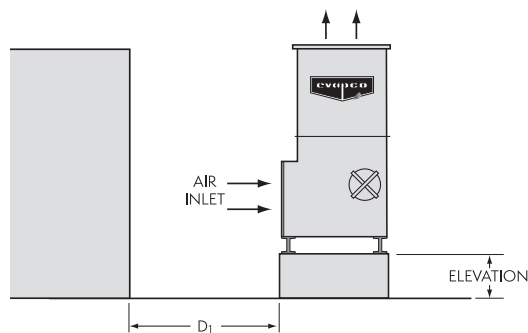
Figure 38 – Installation Next to Wall
